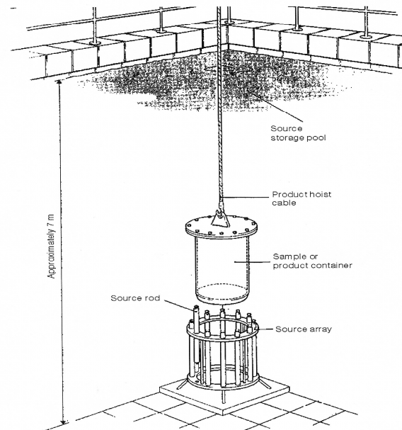
FIG. 2. Category III gamma irradiation facility: Underwater irradiator.
